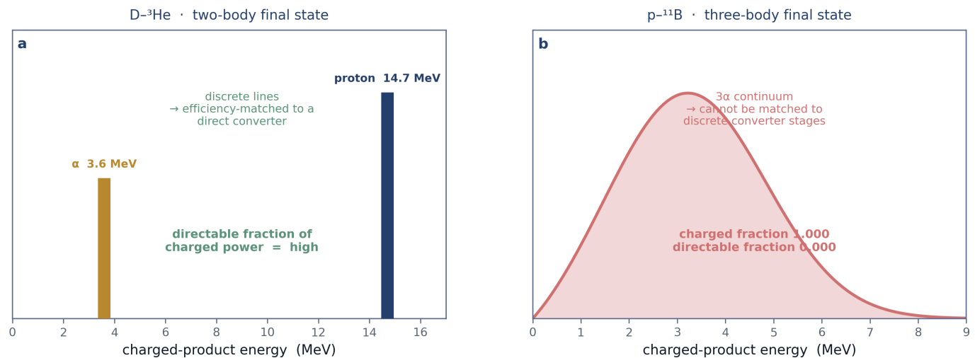
Fig. 3 Any conversion efficiency quoted across two fuels of different final-state multiplicity is wrong on its face (bears on Aegis / MetroVolt $4).
